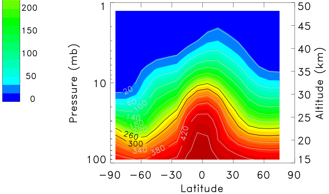
CF 2 Cl 2 (pptv) Model Sept. 1992
