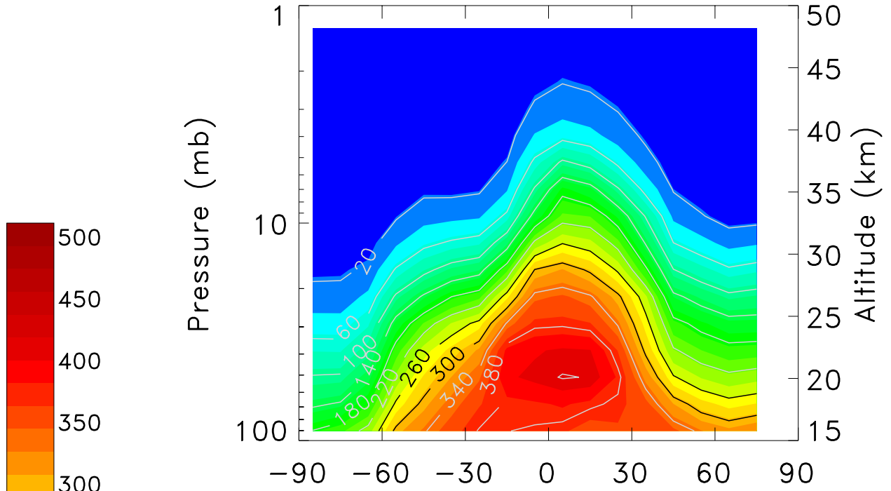
CF 2 Cl 2 (pptv) CLAES v7 Sept. 1992
