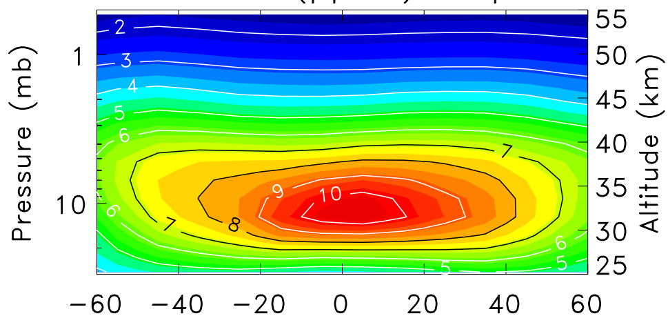
Model Ozone (ppmv) Sept. 1992
