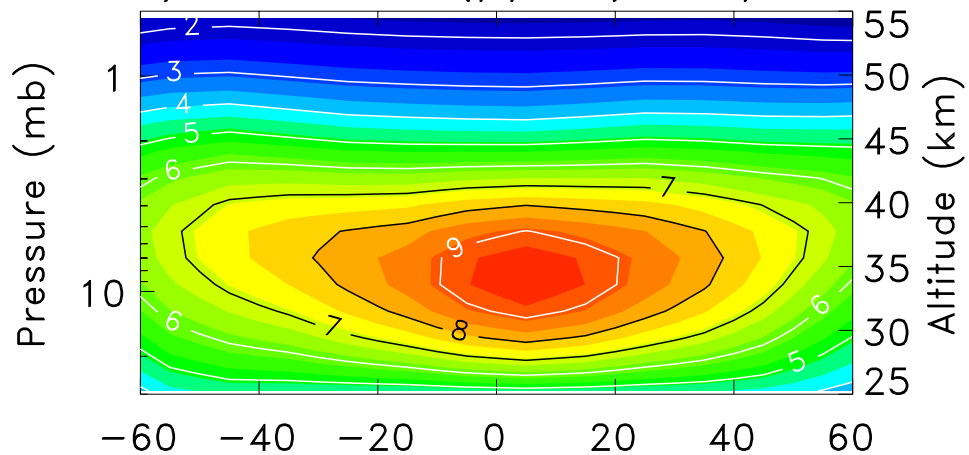
SBUV/2 Ozone (ppmv) Sept. 1992
