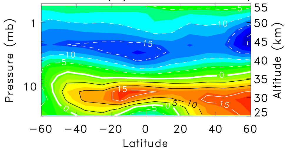
Difference (%) Model - SBUV/2
