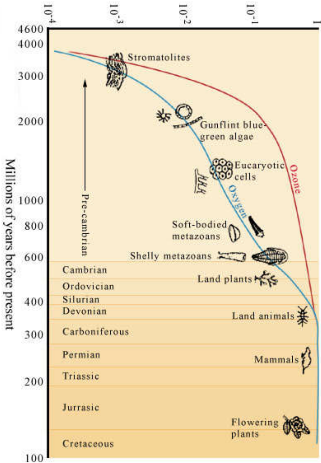
Ground level oxygen concentration or ozone column abundance as fraction of present atmospheric level
