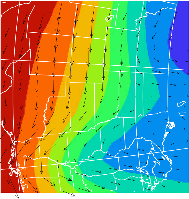
500 hPa Z 12/5/96
