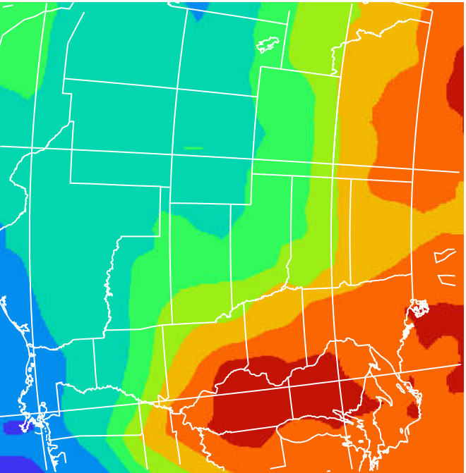
TOMS 12/5/96
