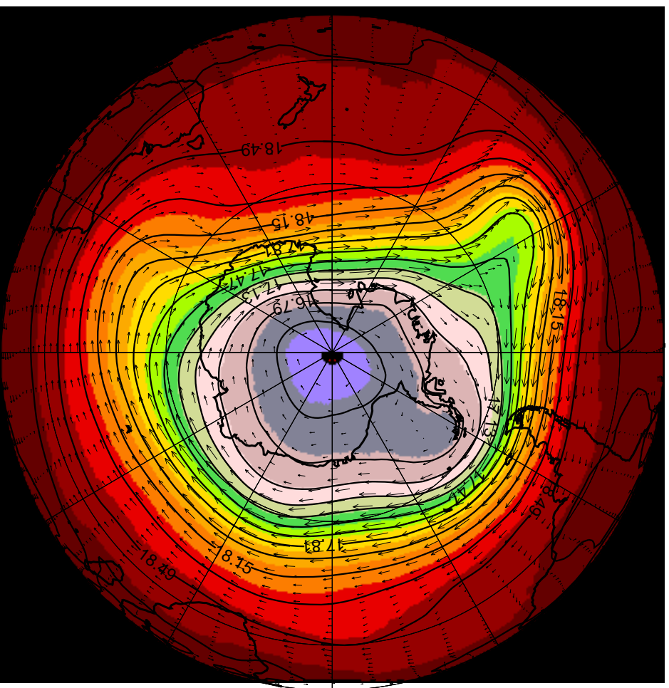
DAO Assimilated Geopotential Height(km) and Wind Vectors(m/s) at 70 hPa on 15 September 1996 at 12 GMT
