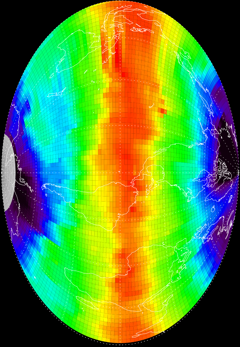
SBUV O 3 @ 15mb
