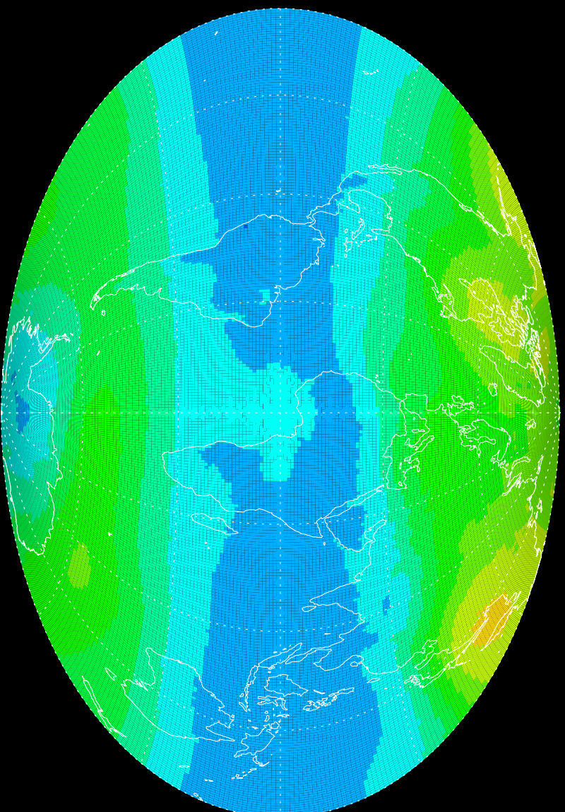
Average TOMS Ozone 1978 – 1993
