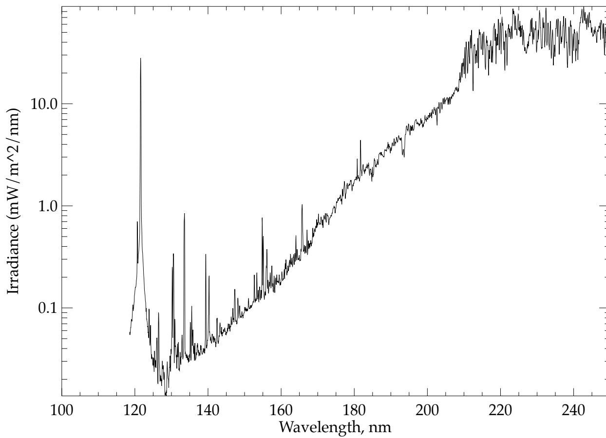
Extraterrestrial Solar Irradiance at 1 A.U.
