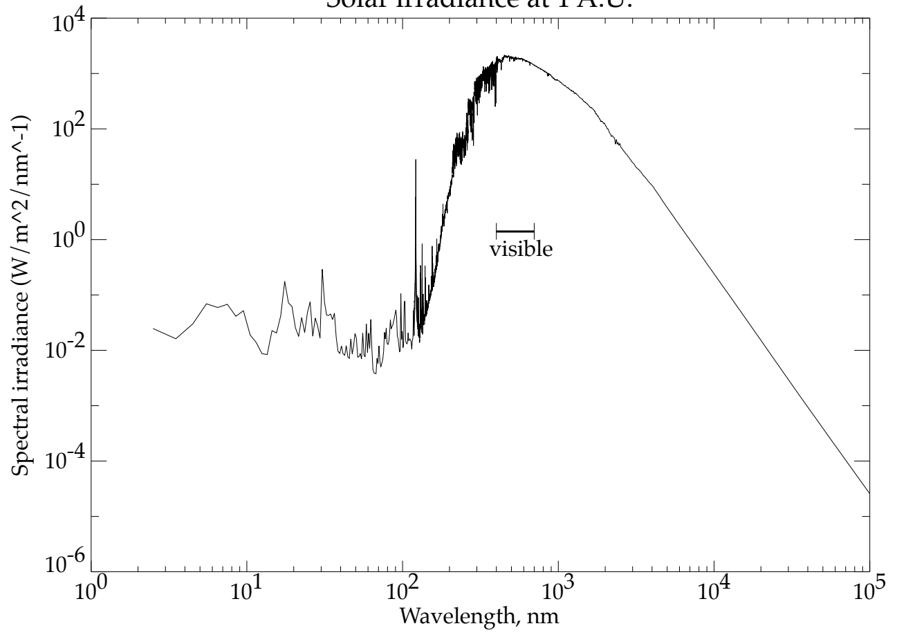
Solar irradiance at 1 A.U.
