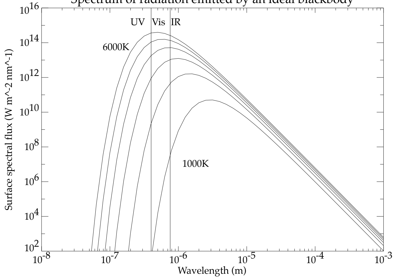
Spectrum of radiation emitted by an ideal blackbody
