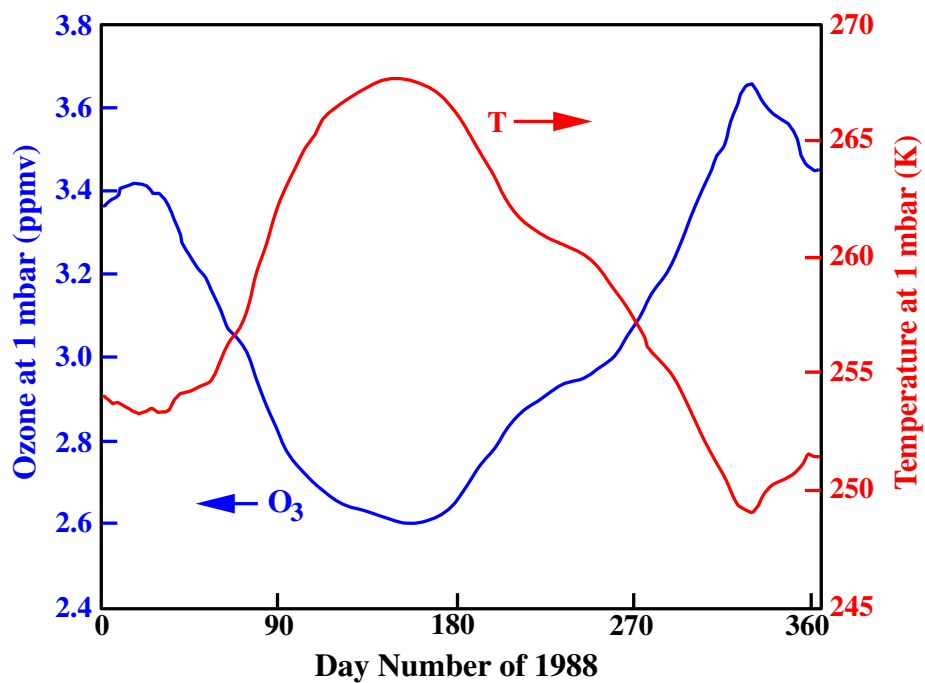
Seasonal variation of ozone and temperature at 1 mbar
