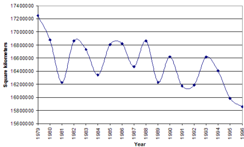
Northern Hemisphere Sea Ice Extent in March
