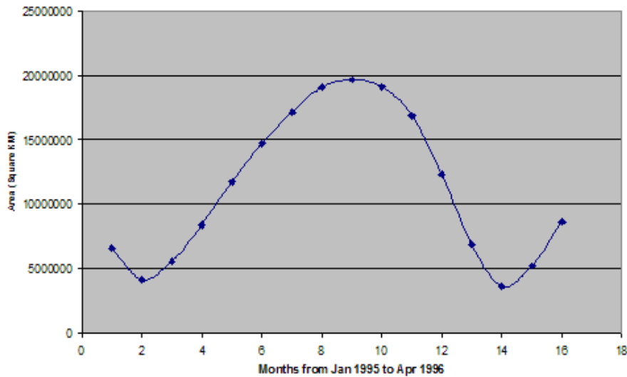
Southern Hemisphere Sea Ice Extent
