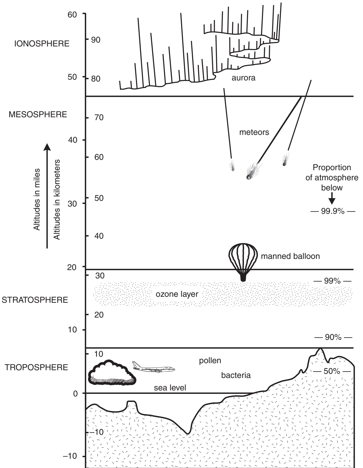
Figure 1.02 Diagram of atmospheric layers
