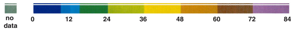
Figure 2.04 Global average albedo for January 1986
