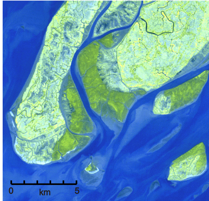
Landsat TM, coastal Bangladesh, 02 Mar 98
