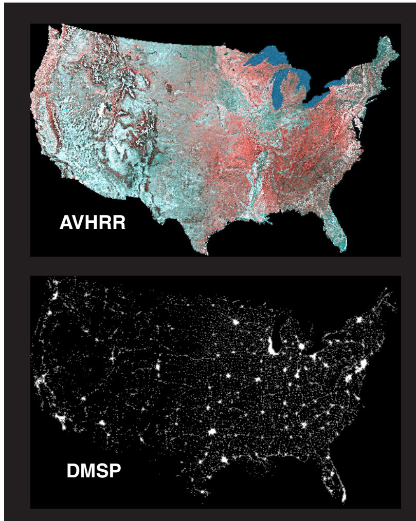
Figure 8.04: Lights of the USA from DMSP with AVHRR reference mosaic
