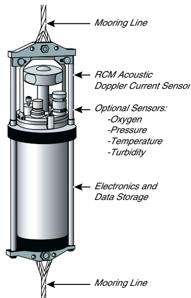
Figure 10.19 An example of a moored current meter, the RCM 9 produced by Aanderaa Instruments. Two components of horizontal velocity are measured by an acoustic current meter, and the directions are referenced to north using an internal Hall-effect compass. The electronics, data recorder, and battery are in the pressure-resistant housing. Accuracy is \pm 0.15 cm/s and \pm 5^\circ . (Courtesy Aanderaa Instruments)
