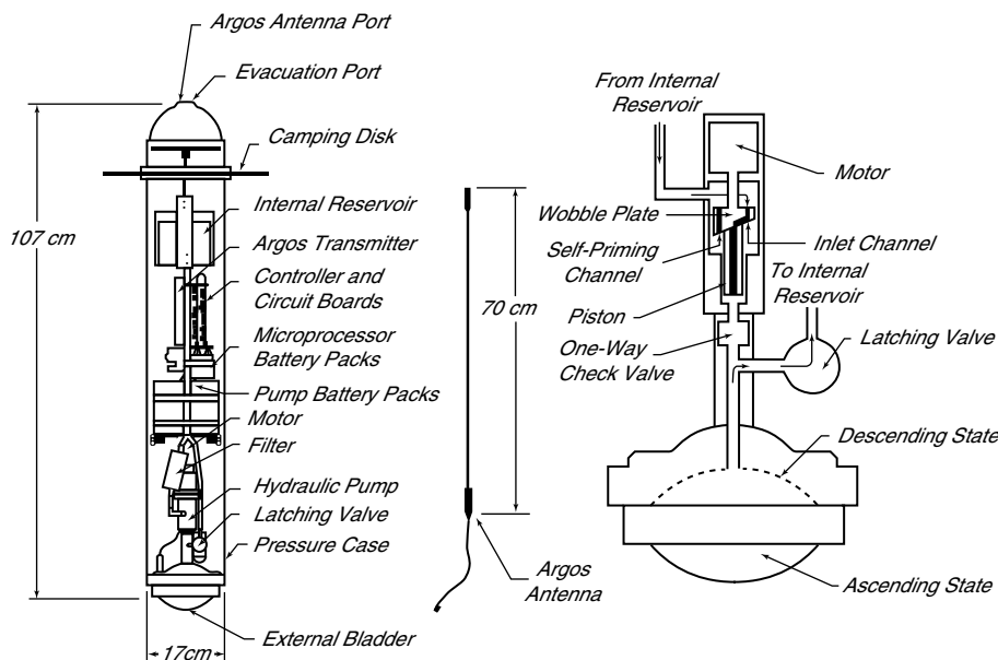
Figure 10.14 The Autonomous Lagrangian Circulation Explorer (ALACE) floats are widely used by the World Ocean Circulation Experiment to measure mid-depth currents. Left: Schematic of the drifter. To ascend, the hydraulic pump moves oil from an internal reservoir to an external bladder, reducing the drifter's density. To descend, the latching valve is opened to allow oil to flow back into the internal reservoir. The antenna is mounted to the end cap. Right: Expanded schematic of the hydraulic system. The motor rotates the wobble plate actuating the piston which pumps hydraulic oil. After Davis et al. (1992).
