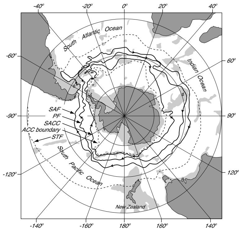
Figure 13.13 Distribution of fronts around Antarctica: STF : Subtropical Front; SAF : Subantarctic Front; PF : Polar Front; SACC : Southern Antarctic Circumpolar Front. Shaded areas are shallower than 3 km. From Orsi (1988).
