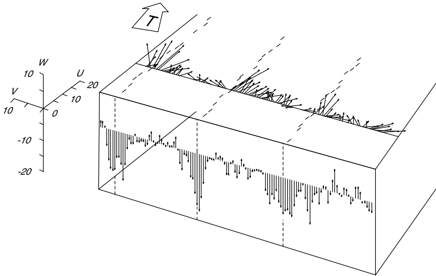
Figure 9.8 A three-dimensional view of the Langmuir circulation at the surface of the Pacific observed from the Floating Instrument Platform FLIP. The heavy dashed line on the sea surface indicate lines of convergence marked by cards on the surface. Vertical arrows are individual values of vertical velocity measured every 14 seconds at 23 m depth as the platform drifted through the Langmuir currents. Horizontal arrows, which are drawn on the surface for clarity, are values of horizontal velocity at 23 m. The broad arrow gives the direction of the wind. After Weller et al. (1985).
