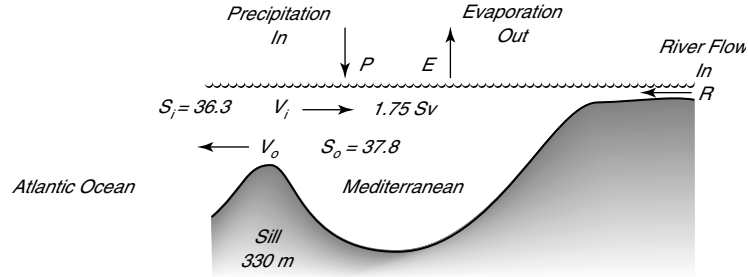
Figure 7.1 Schematic diagram of flow into and out of a basin. After Pickard and Emery (1990: 65).
