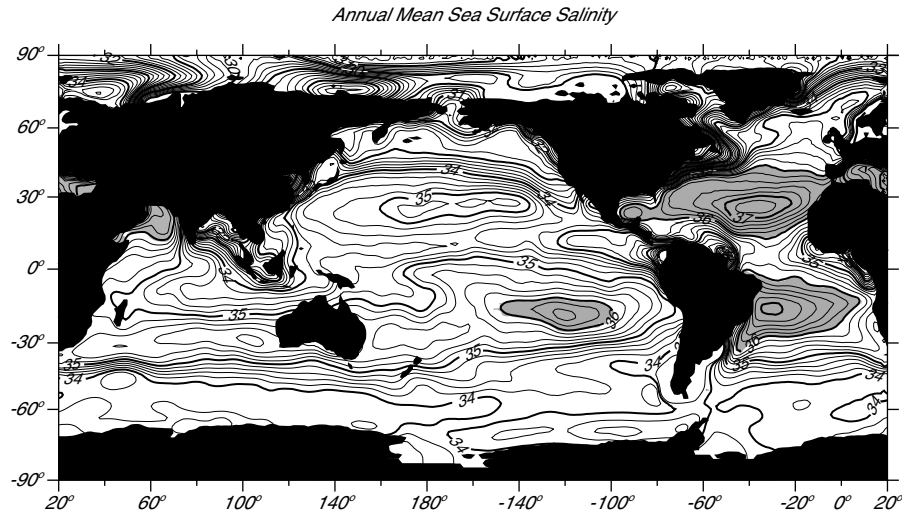
Figure 6.4 Mean sea-surface salinity. Contour interval is 0.25. Shaded areas exceed a salinity of 36. From Levitus (1982).
