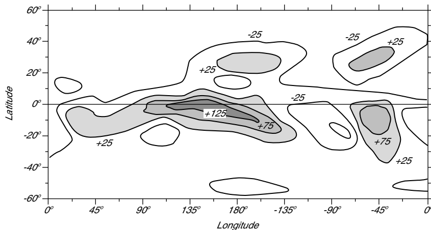
Figure 14.1 Average diabatic heating between 700 and 50 mb in the atmosphere during December, January and February calculated from ECMWF data for 1983–1989. Most of the heating is due to the release of latent heat by rain. After Webster et al. (1992).
