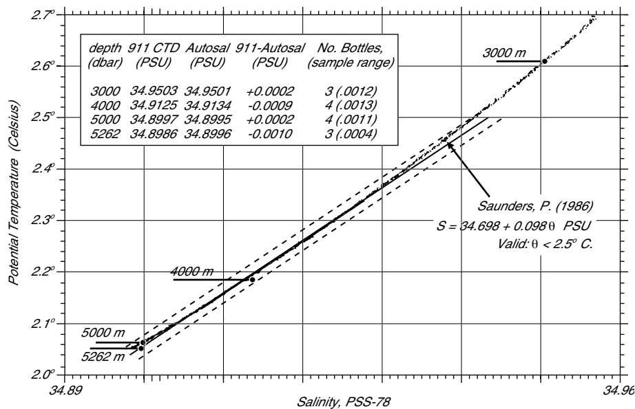
Figure 6.15. Results from a test of the Sea-Bird Electronics 911 Plus CTD in the North Atlantic Deep Water in 1992. Data were collected at 43.17° N and 14.08° W from the R/V Poseidon. From Sea-Bird Electronics (1992).
