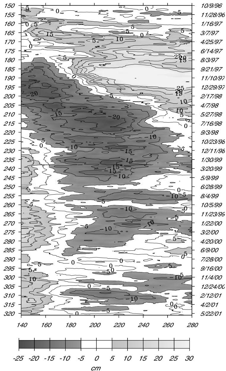
Figure 10.6 Time-longitude plot of sea-level anomalies in the Equatorial Pacific observed by Topex/Poseidon. Warm anomalies are light gray, cold anomalies are dark gray. The anomalies are computed from 10-day deviations from a three-year mean surface from 3 Oct 1992 to 8 Oct 1995. The data are smoothed with a Gaussian weighted filter with a longitudinal span of 5^\circ and a latitudinal span of 2^\circ . The annotations on the left are cycles of satellite data. From Center for Space Research, University of Texas.
