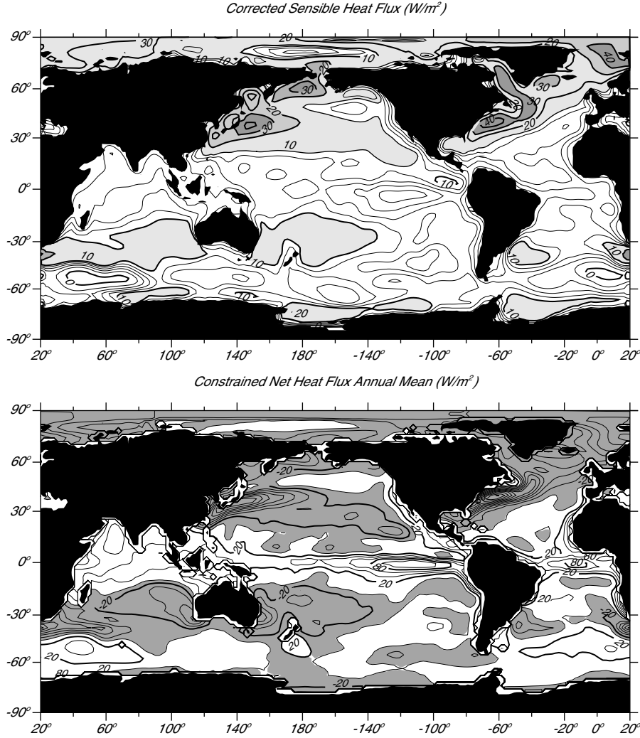
Figure 5.10 Annual-mean upward sensible heat flux Q_S (top) and constrained, net, downward heat flux (bottom) through the sea surface in \text{W/m}^2 calculated by DaSilva, Young, and Levitus (1995) using the COADS data set from 1945 to 1989. Contour interval is 2 \text{W/m}^2 (top) and 20 \text{W/m}^2 (bottom).
