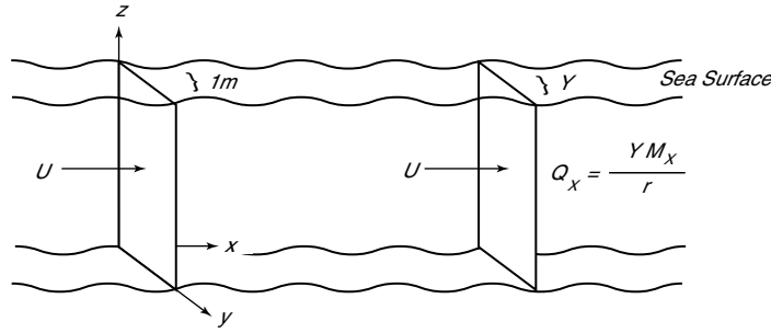
Figure 9.6 Sketch for defining Left: mass transports, and Right: volume transports.
