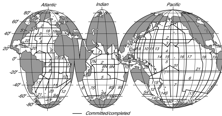
Figure 2.5 World Ocean Circulation Experiment: Tracks of research ships making a one-time global survey of the oceans of the world. From World Ocean Circulation Experiment.
