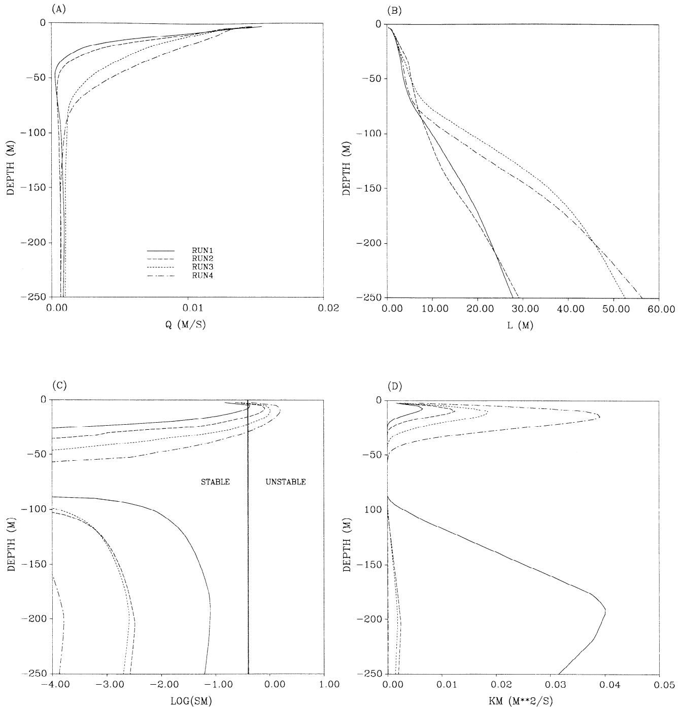
Figure 10. Vertical profiles of the turbulence parameters on September 30 averaged over the northeast Atlantic region: (a) the turbulence velocity magnitude q , (b) the turbulence length scale \ell , (c) log of the stability factor S_M , and (d) the vertical diffusivity coefficient K_M . Run 1, run 2, run 3, and run 4 are indicated by solid, dashed, dotted and dash-dotted lines, respectively.
