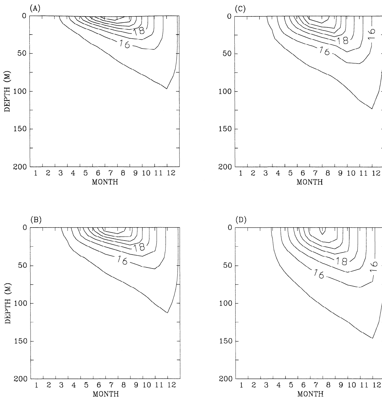
Figure 6. Area-averaged and monthly averaged temperatures as a function of depth and time for the northeast Atlantic region: (a) run 1, (b) run 2, (c) run 3, and (d) run 4. The contour interval is 1°C.
