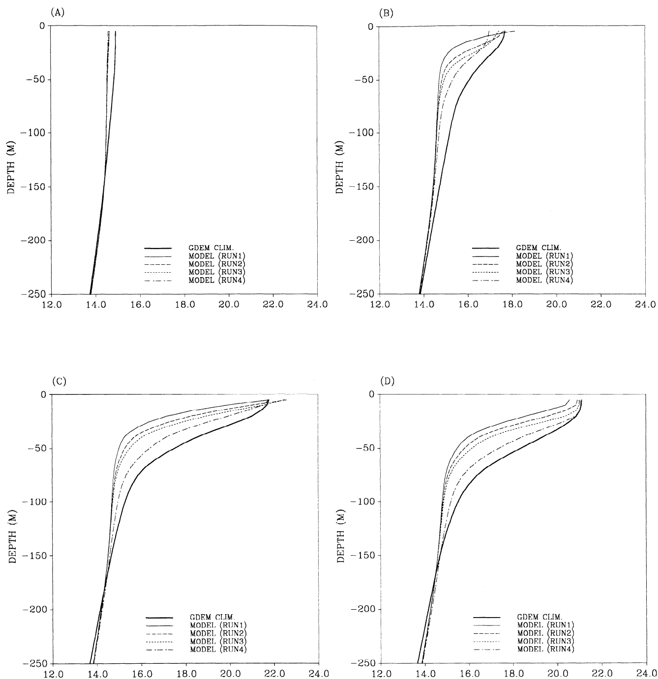
Figure 9. Vertical profiles of temperature averaged over the northeast Atlantic area indicated in Figure 1 for (a) March 30, (b) May 30, (c) July 30, and (d) September 30. Solid heavy lines are obtained from the GDEM climatology; model calculations for run 1, run 2, run 3, and run 4 are indicated by thin solid, dashed, dotted and dash-dotted lines, respectively.
