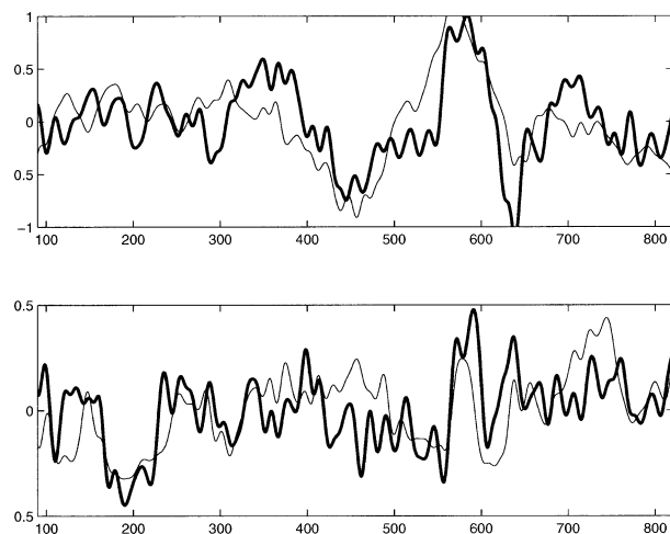
FIG. 8. (top) First and (bottom) second modes of observed (heavy lines) and model (light lines) currents. The time is referenced to 1 Jan 1997.
