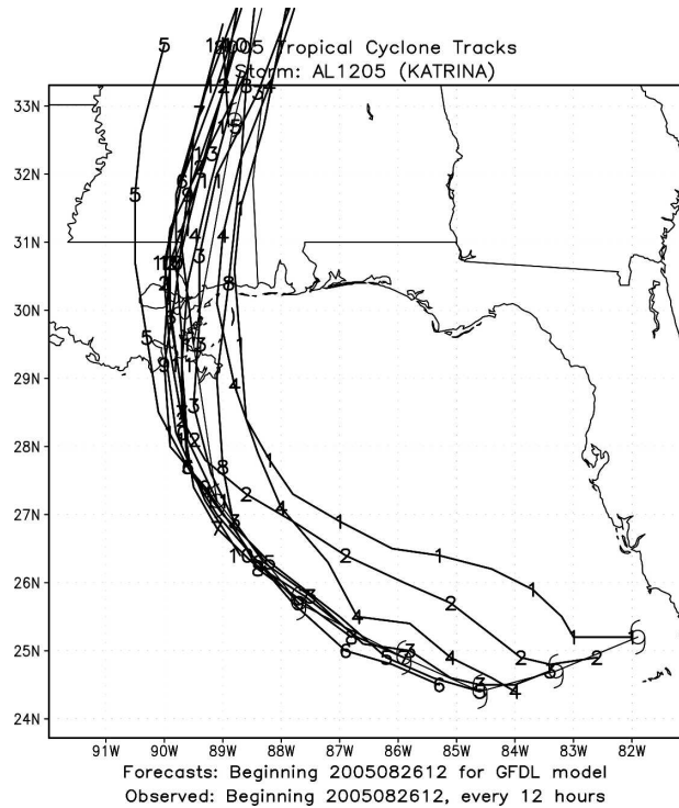
FIG. 12. Composite of all GFDL forecasts for Hurricane Katrina, starting on or after 1200 UTC 26 Aug. The observed track is noted by the black line with the observed position at 12-h intervals denoted by the hurricane symbol.
