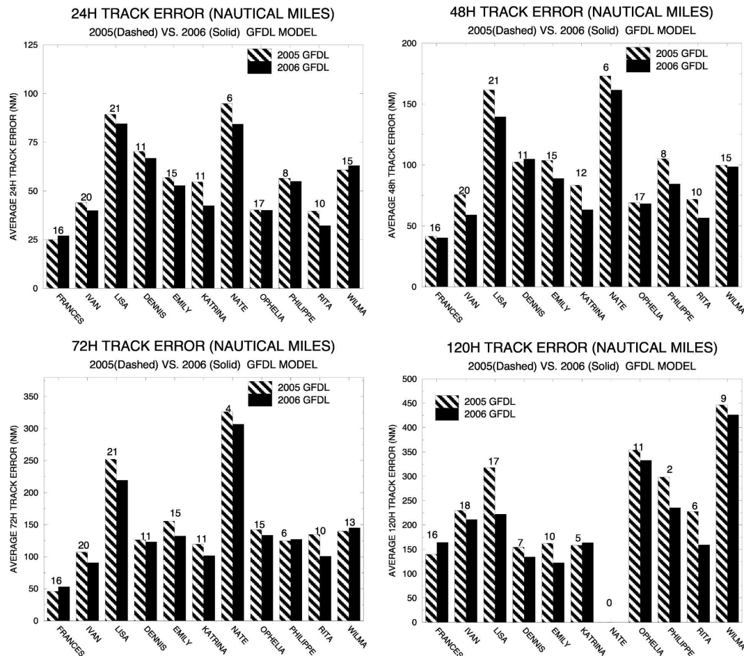
FIG. 20. Distribution by storm of the average track error at 24, 48, 72, and 120 h for the forecasts run with the 2005 version of the GFDL model and the version made operational in 2006. Cases selected were from the 2004 and 2005 hurricane season. Total number of forecasts run for each storm is indicated.
